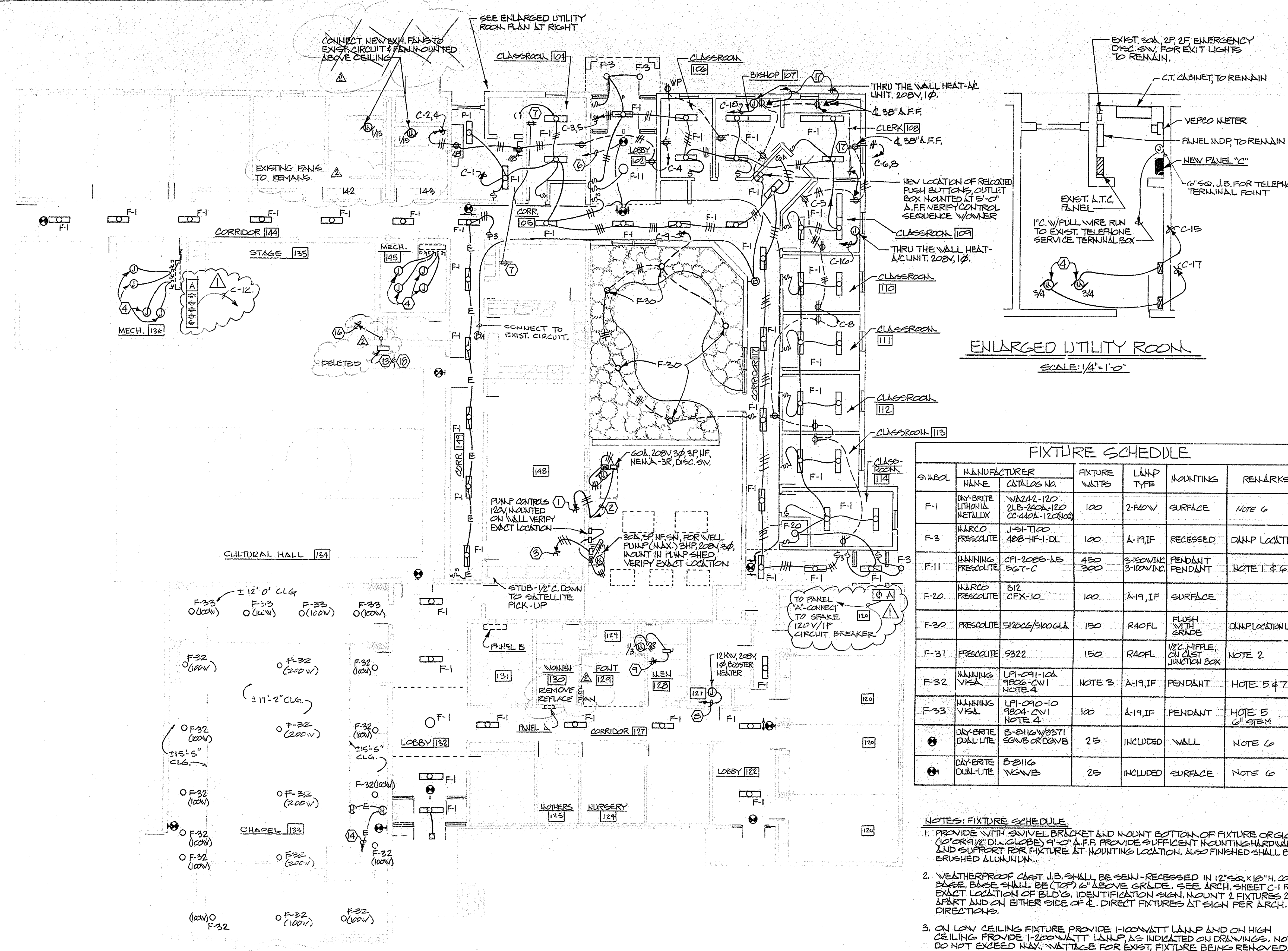
ELECTRICAL NEW WORK FLOOR PLAN SCALE: 1/8" = 1'-0"
