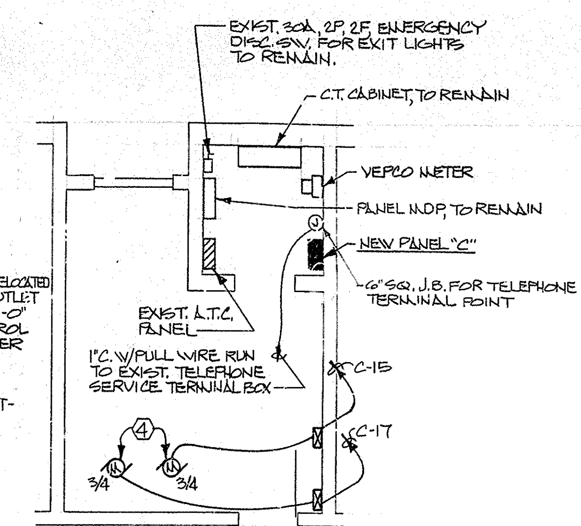
ENLARGED UTILITY ROOM SCALE: 1/4" = 1'-0"
